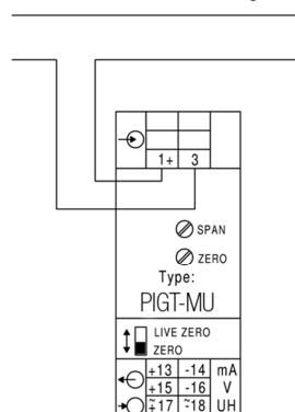
DC-Strommessung DC-current measuring
